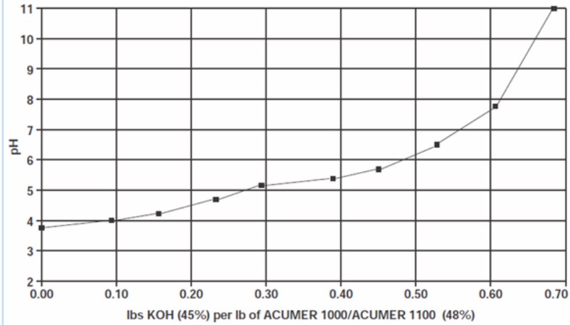
FIGURE 2b — NEUTRALIZATION OF ACUMER 1000/ACUMER 1100 (PRODUCT) WITH KOH (45%)
