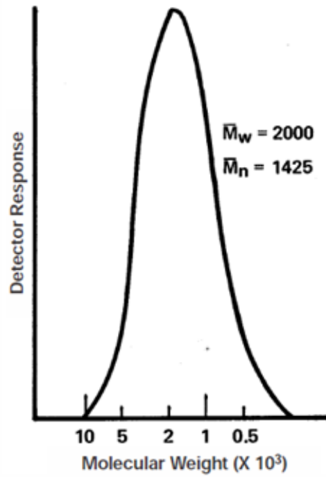
FIGURE 1 — MOLECULAR WEIGHT DISTRIBUTION FOR ACUMER 1000/ACUMER 1020 BY AQUEOUS GPC
