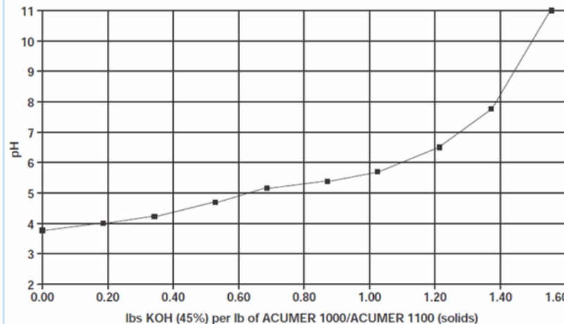
FIGURE 2d — NEUTRALIZATION OF ACUMER 1000/ACUMER 1100 (SOLIDS) WITH KOH (45%)
