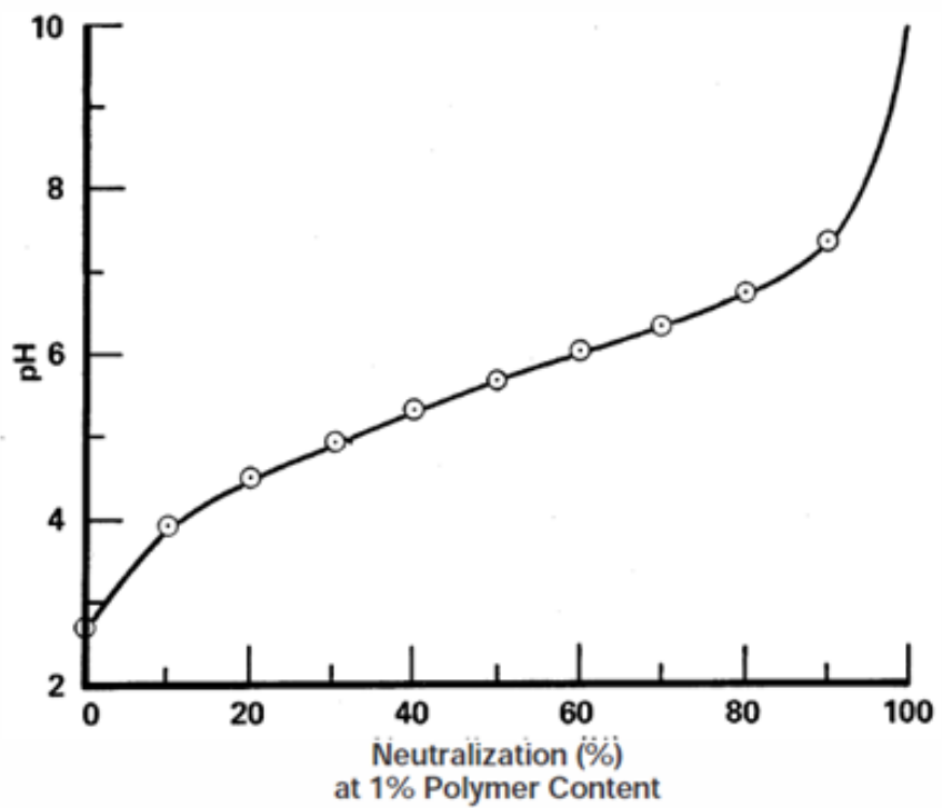
FIGURE 2a — NEUTRALIZATION OF ACUMER POLYMERS
