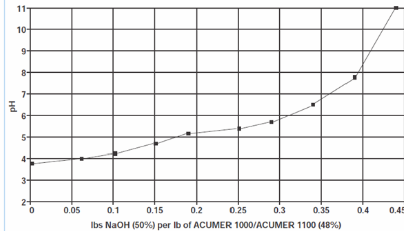
FIGURE 2c — NEUTRALIZATION OF ACUMER 1000/ACUMER 1100 (PRODUCT) WITH NaOH (50%)
